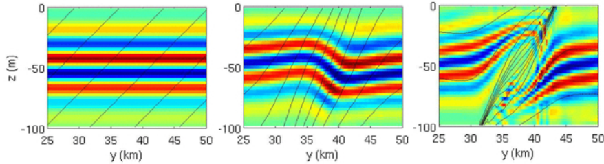
Fig. 18 Cross-sections of the y -component of the wave velocity field (color) and isopycnals (contours) at, from left to right, t = 0, 5, and 9 inertial periods into a numerical simulation of a NIW with initially no horizontal wavenumber in a front undergoing frontogenesis. The sections were made at x = 18.75 km in a region where the eddy-driven strain field is frontogenetic. The color scale is the same in each panel and spans velocities between -0.01 and 0.01 \text{ m s}^{-1} . The contour interval for the density is 0.08 \text{ kg m}^{-3} in each panel.
