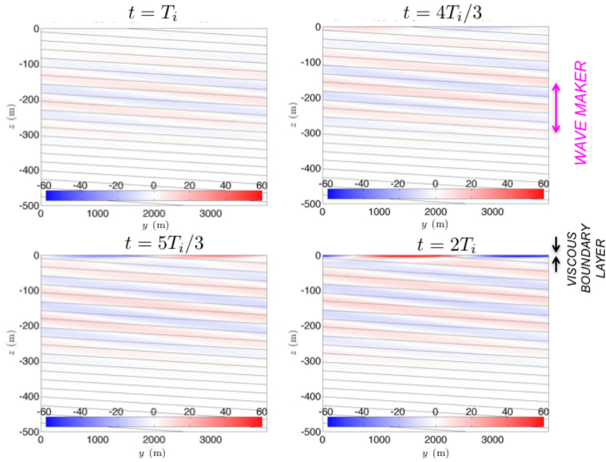
Fig. 7 Snapshots of the along-front component of the vorticity (normalized by f ) of an inertial wave (i.e. with frequency \omega = f ) at 1, 4/3, 5/3, and 2 inertial periods in a front with isopycnals in black from a linear numerical simulation. Note that the flow is invariant in the along-front x -direction and the cross-front coordinate is y . The wave is forced by a wave maker at the depth indicated by the magenta arrow to the right that generates an upward propagating inertial wave packet. As the waves hit the surface, they experience a critical reflection and generate a thin viscous boundary layer.
