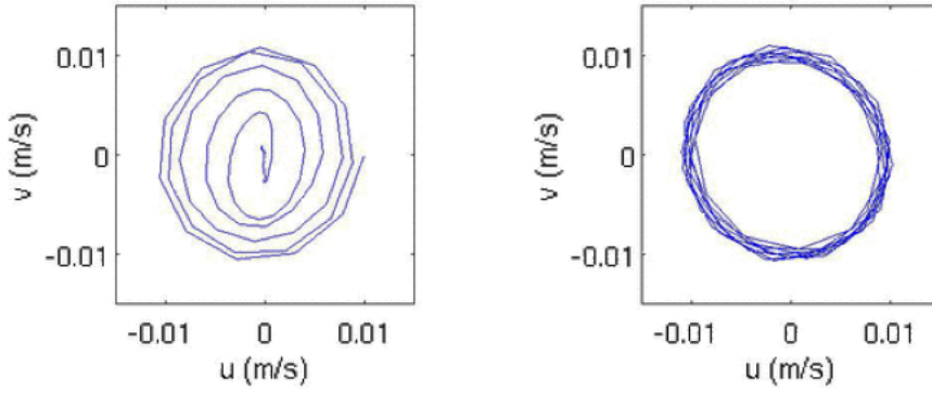
Fig. 15 Hodographs of the wave velocity at mid-depth ( z = -50 m), y = 37.5 km, and traced between 0 and 8 inertial periods from the numerical simulation used to study NIWs in a front undergoing frontogenesis. The hodograph on the left (right) was made at x = 18.75 km ( x = 56.25 km) in a region where the eddy-driven strain field is frontogenetic (frontolytic).
