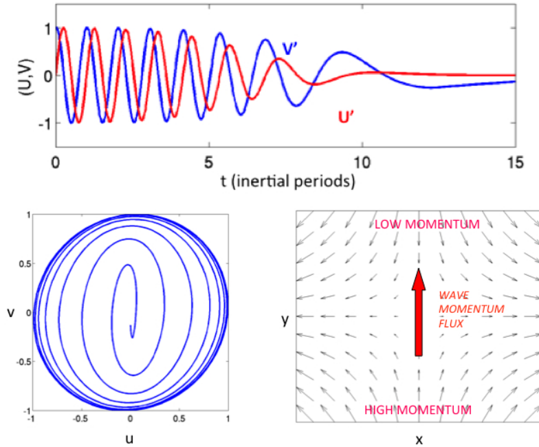
Fig. 11 Top panel: Change in the along-front, u' (red), and cross-front, v' (blue), components of the velocity (both normalized by the initial speed of fluid velocity of the wave) of a near-inertial wave in the background flow undergoing frontogenesis shown in Fig. 10. The time series is made in a frame moving with the background flow, therefore the lengthening of the wave period reflects changes in the intrinsic rather than Eulerian frequency of the wave. Bottom left panel: a hodograph of the velocities in the top panel (from t = 0 to 15 inertial periods) reveals how a near-inertial wave in a front undergoing frontogenesis experiences a change in polarization relation, transitioning from being circularly polarized to rectilinear in the cross-front, y -direction. In the process, the wave induces a momentum flux that is down the gradient in momentum associated with the eddy-driven strain field whose velocity (\alpha x, -\alpha y) is shown in plan view in the bottom right.
