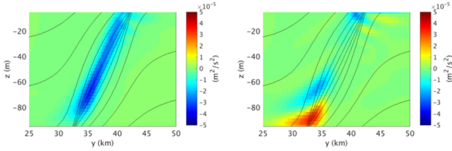
Fig. 17 Left: cross-section of the amount of KE removed from the ageostrophic flow by the NIWs, i.e. \int AGSPdt , eight inertial periods into the simulation used to study NIWs in a front undergoing frontogenesis. Right: cross-section of the amount of KE removed from the frontal geostrophic flow by the NIWs, i.e. \int GSPdt , eight inertial periods into the simulation. The color scale in both panels is the same as in Figure 16 and both quantities are evaluated at x = 18.75 km in a region where the eddy-driven strain field is frontogenetic. Isopycnals are contoured with an interval of 0.08 \text{ kg m}^{-3} in both panels.
