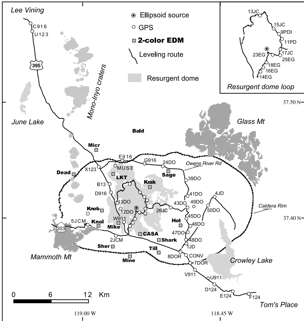
Fig. 1. Map of Long Valley caldera geodetic networks.
