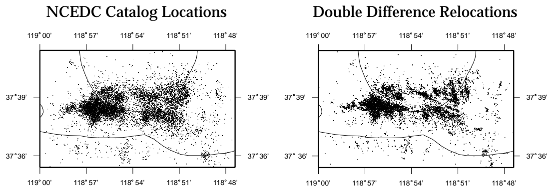
Figure 2.3 - July 1997–January 1998 Long Valley caldera seismicity before (left) and after (right) double-difference relocation (Waldhauser and Ellsworth, 2000) using P-phase catalog arrival times obtained by the Northern California Earthquake Data Center. (NCEDC)
